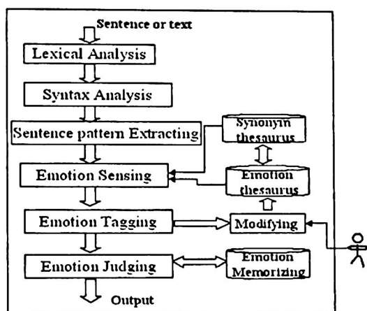
Fig.1 Flow chart of the emotion classification model
